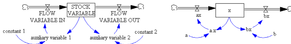
Figure 5.1: A basic stock/flow diagram with a stock, a flow, an auxiliary variable and a constant
