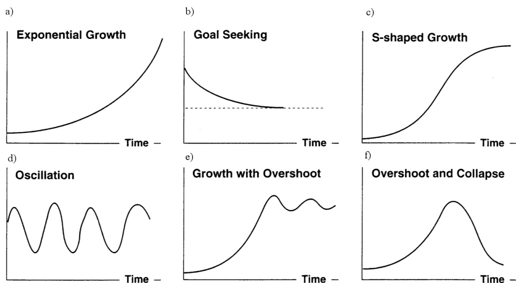
Figure 14.1: Modes of behaviours of simple dynamic systems as in (Stermann, 2000, p108)
