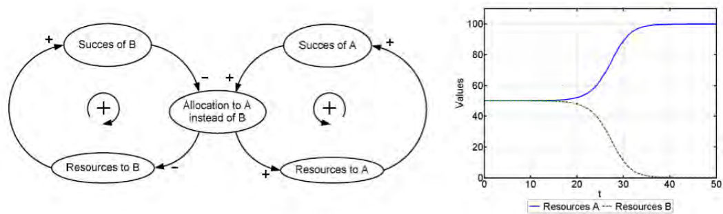
(b) AD of the success to the successful archetype and possible behavior
