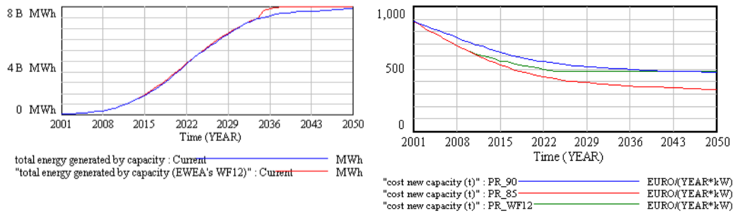
Figure 22.5: Left-hand side: Total energy generated by capacity as in the Wind Force 12 report (red curve) and as calculated in the corrected model (blue curve). Right-hand side: The impact on the cost of new capacity ( t )[€/kW] of the changing progress ratio of the Wind Force 12 report compared to two constant progress ratios of 85% and 90%.
