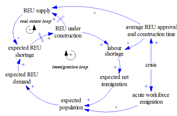
(a) CLD of the RE crisis
